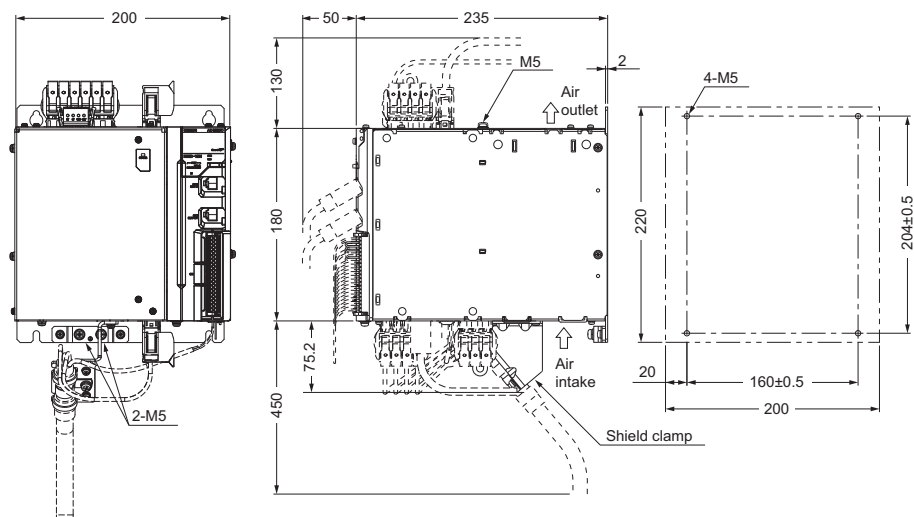
Mounting dimensions
