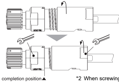
completion position ▲ *2 When screwing up the cap by large size tool, it may cause damage.
